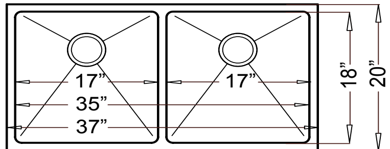
Product Diagram (Shown with “Radial” corners)
