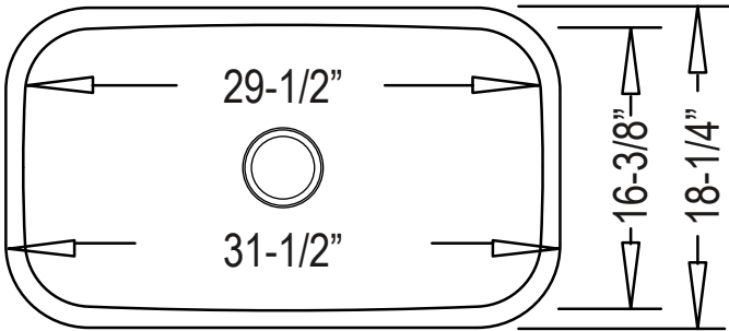
Product Diagram
