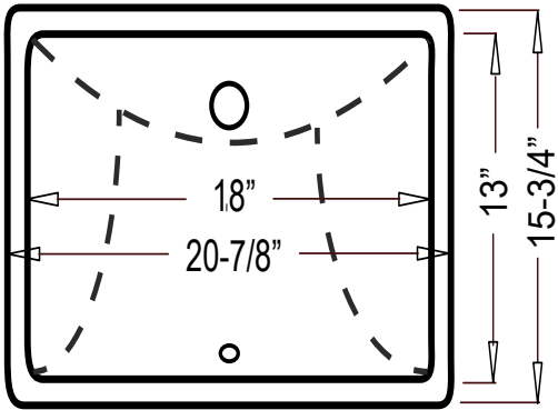
Product Diagram
