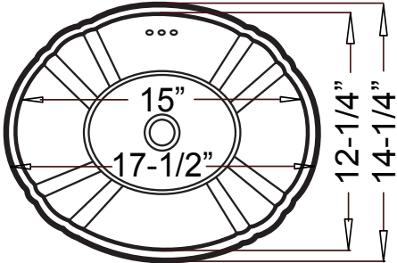
Product Diagram
