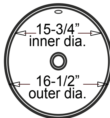
Product Diagram
