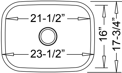
Product Diagram
